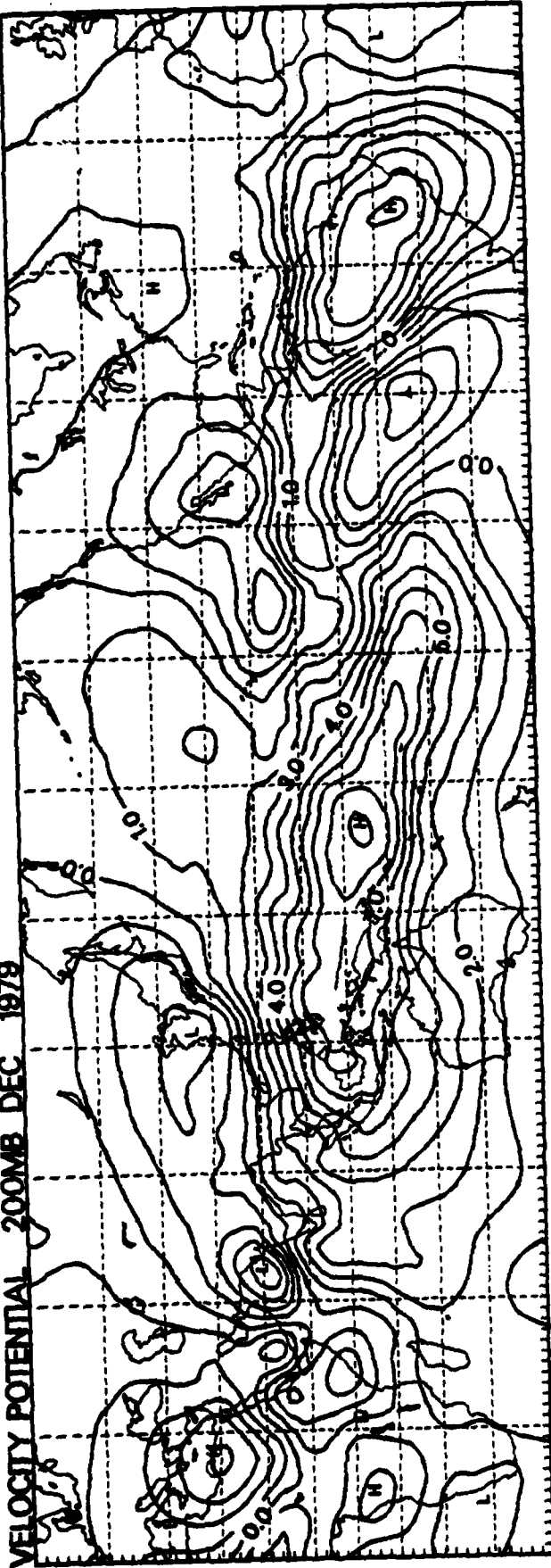
VELOCITY POTENTIAL 200MB DEC 1979
